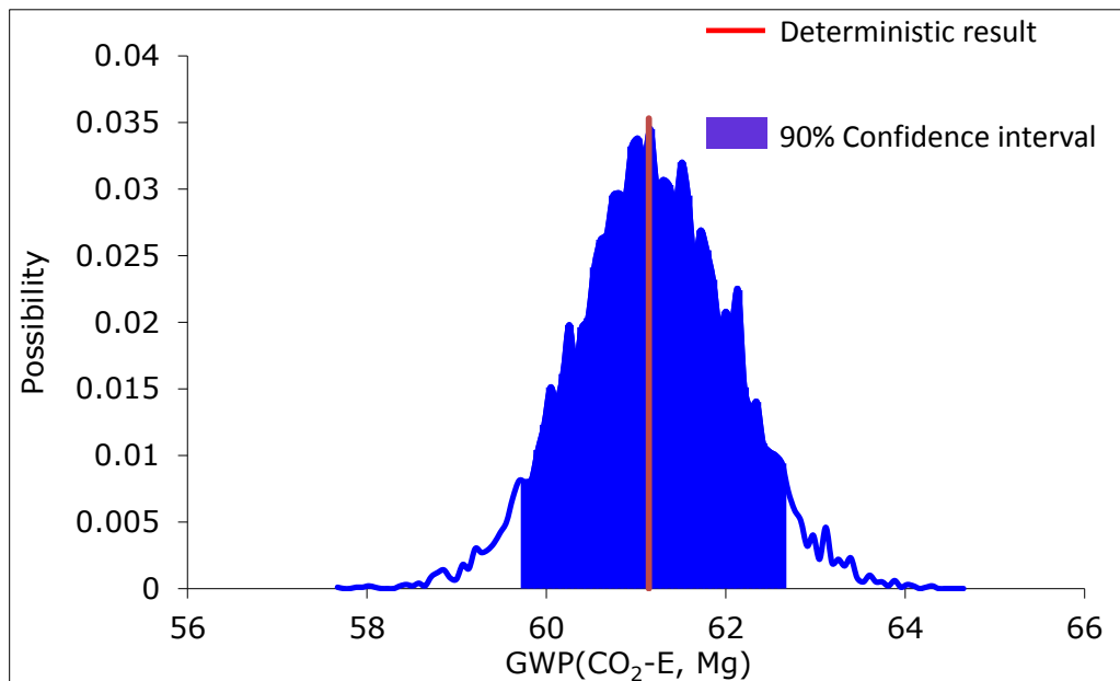
Figure 25 Probability density of GWP from transportation, WA-PCC
